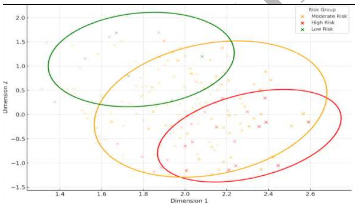
Figure 3: Multiple Correspondence Analysis (MCA) Biplot Showing Risk Groups: the High Risk group (in red); the Moderate Risk group (in orange) and the Low Risk group (in green).
