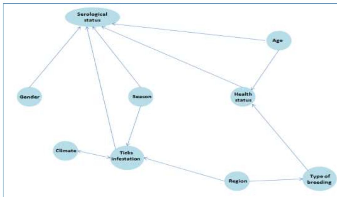
Figure 2 : Directed Acyclic Graph (DAG) representing hypothesized causal pathways influencing seropositivity.
