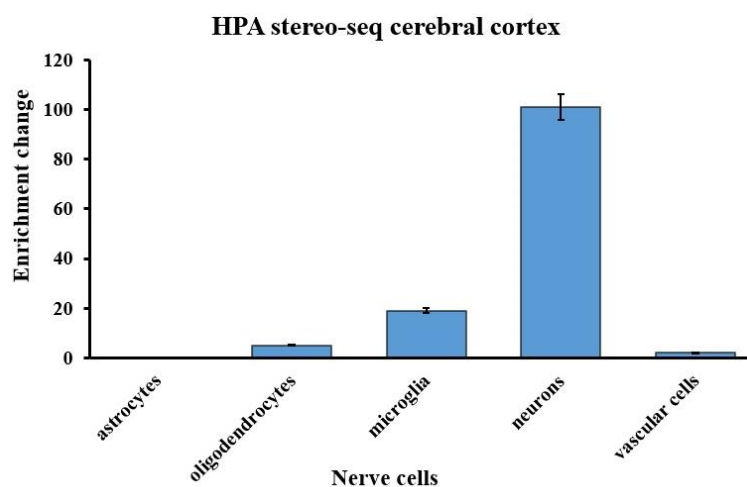
Fig. 4 Quebrachamine protein expression in nerve cells. HPA stereo-seq cerebral cortex associated with Quebrachamine in nerve cells. In this graph, each bar represents the number per million copies in each cell-type mask.
