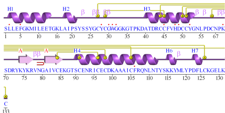
Fig. 9 Calcium-independent PLA2 (iPLA2) protein.
