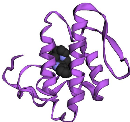
Fig. 10 Docking of Rhazyaminine on Calcium-independent PLA2 (iPLA2) protein.
