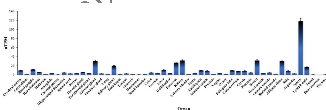
Fig. 5 Changes in Quebrachamine protein expression under the influence of the ACRA4 gene. Changes in Quebrachamine protein expression under the influence of the ACRA4 gene. For genes with low expression levels, expression data in cell clusters are evaluated to produce normalized transcripts per million by cell type, which is indicated by the (nTPM) index.
