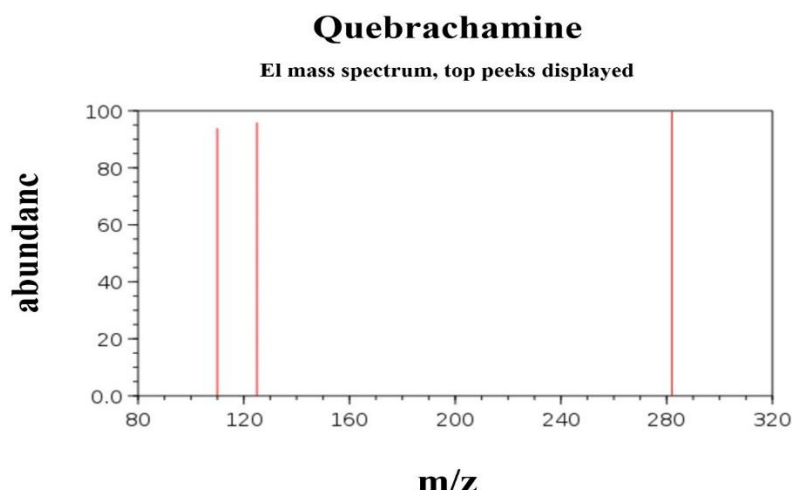
Fig. 6 GC-MS results on Quebrachamine protein. GC-MS results on Quebrachamine protein. m/z (mass-to-charge ratio): In mass spectrometry the ratio of an ion's mass ( m ) in atomic mass units (amu) to its formal charge ( z ).
