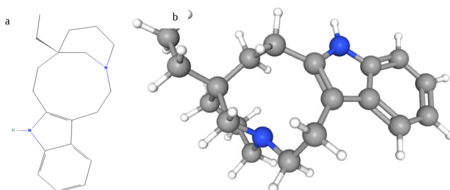
Fig. 1 2D (a) and 3D (b) structures of Quebrachamine protein.
