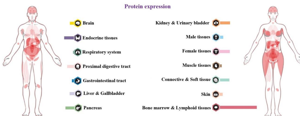
Fig. 3 Quebrachamine protein expression in different organs of the human body. Quebrachamine protein expression in different organs of the human body. Each bar represents the highest expression score found in a particular group of tissues. Protein expression scores are based on the best estimate of true protein expression.
