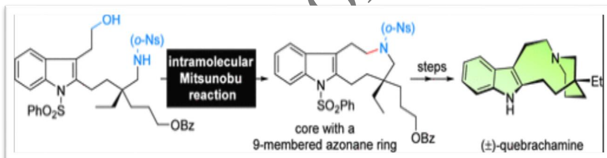
Fig. 2 Total synthesis of Quebrachamine and Kopsiyunnanine D [19].
