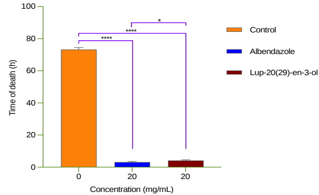
Fig. 7 Comparison of the survival of R. echinobothrida in culture with those treated with albendazole and lup-20(29)-en-3-ol from A. oleracea using one-way ANOVA and Turkey's multiple comparison test; n = 9 ; **** p < 0.0001 ; * p < 0.05 .
