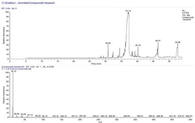
Fig. 6 GC-MS chromatogram and spectra of a compound isolated from A. oleracea . Structure of lup-20(29)-en-3-ol as generated from the NIST chemical library.
