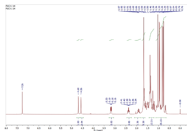
Fig. 3 1 H NMR spectrum at 400 MHz in CDCl 3 of a compound isolated from A. oleracea .
