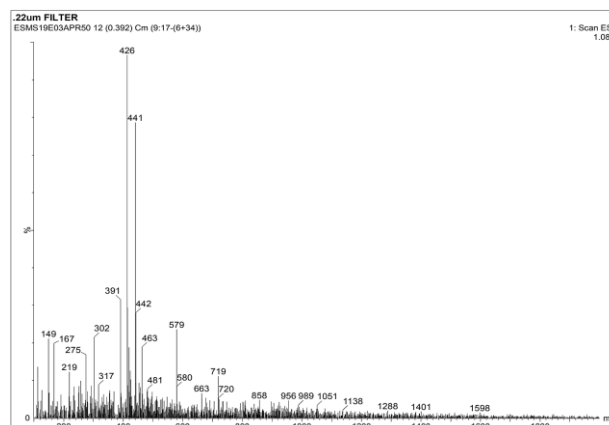
Fig. 2 APCI-ESI-HRMS mass spectra of a compound isolated from A. oleracea .
