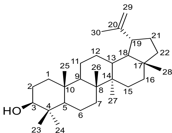
Fig. 1 Structure of lup-20(29)-en-3-ol.
