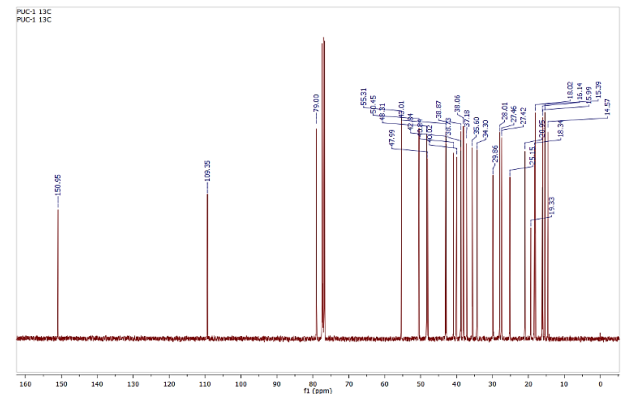
Fig. 4 13 C NMR spectra at 100 MHz in CDCl 3 of a compound isolated from A. oleracea .
