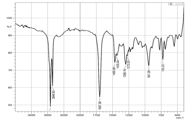
Fig. 5 FTIR spectra of a compound isolated from A. oleracea .
