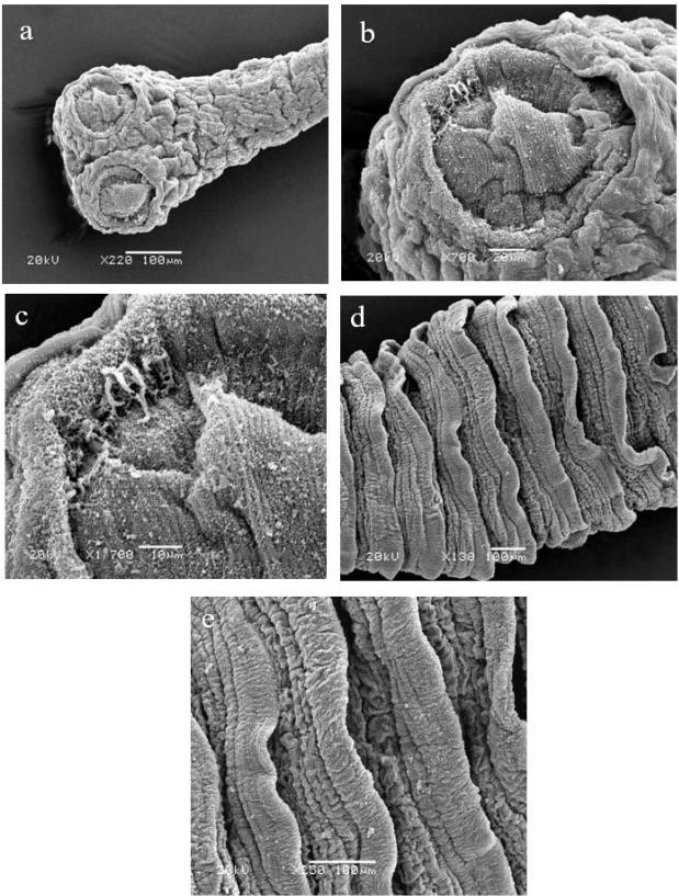
Fig. 8 Scanning electron micrographs of different body parts of poultry tapeworm treated with a compound isolated from A. oleracea . (a) Scolex and neck region showing rostellum (slight depression) at the tip and two oval suckers. (b) One sucker focussed to show removal of the tegument and the spines. (c) Magnification of the same sucker showing almost complete loss of the spines except for four of them (white fang-like structures) on the top. (d) The main body showing a chain of body segments, and the body surface is abnormally folded. (e) Enlarged view of the mature segment indicating heavy tegumental folds and several tissue debris and warts.
