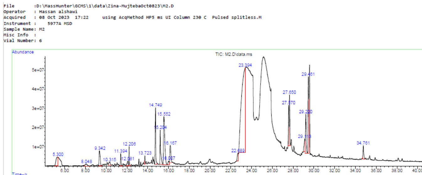
Fig. 1 GC-MS Chromatogram of P. khinjuk Fruit Oil Extract
