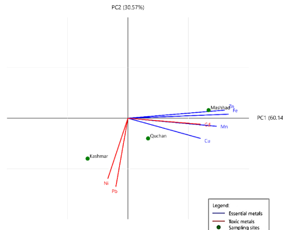
Fig. 1 PCA biplot of heavy metal relationships and market distribution patterns in lavender samples from Khorasan Razavi region, Iran. Loading vectors show the distribution of seven analyzed metals (Fe, Zn, Cu, Mn, Cd, Pb, Ni) across the first two principal components (PC1: 60.14%, PC2: 30.57%, total variance explained: 90.71%). Essential metals are shown in blue vectors, potentially toxic metals in red vectors, and market locations as green circles. The data represents mean values from 18 composite samples collected from three major medicinal plant markets ( n=6 per market).
