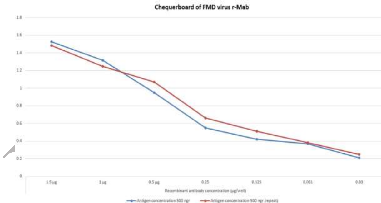
Figure3. ELISA absorbance results in a chequerboard pattern with different concentrations of recombinant antibody (X axis) and fixed virus antigen 0.5 µg/well (Y axis), 1/10 dilution of secondary BRS antibody and also 1:10000 dilution of Hrp-conjugated tertiary antibody were used. Finally, Optimum concentration of 0.4 µg/well of r-mAb antibody was selected for next Capture ELISA tests.
