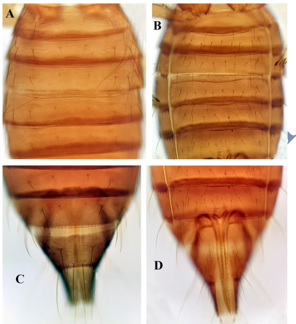
Fig. 2. Thrips mazandaran sp. n., Holotype female: A. Abdominal tergites II–VI; B. Abdominal sternites II–VII; C. Abdominal tergites VII–X, showing poteromarginal comb, and two pairs of CPS on tergite IX; D. Abdominal sternite VI & ovipositor.
