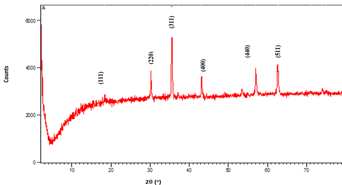
Fig. 2 XRD pattern of SNPs GQD@ \beta -cyclocital
