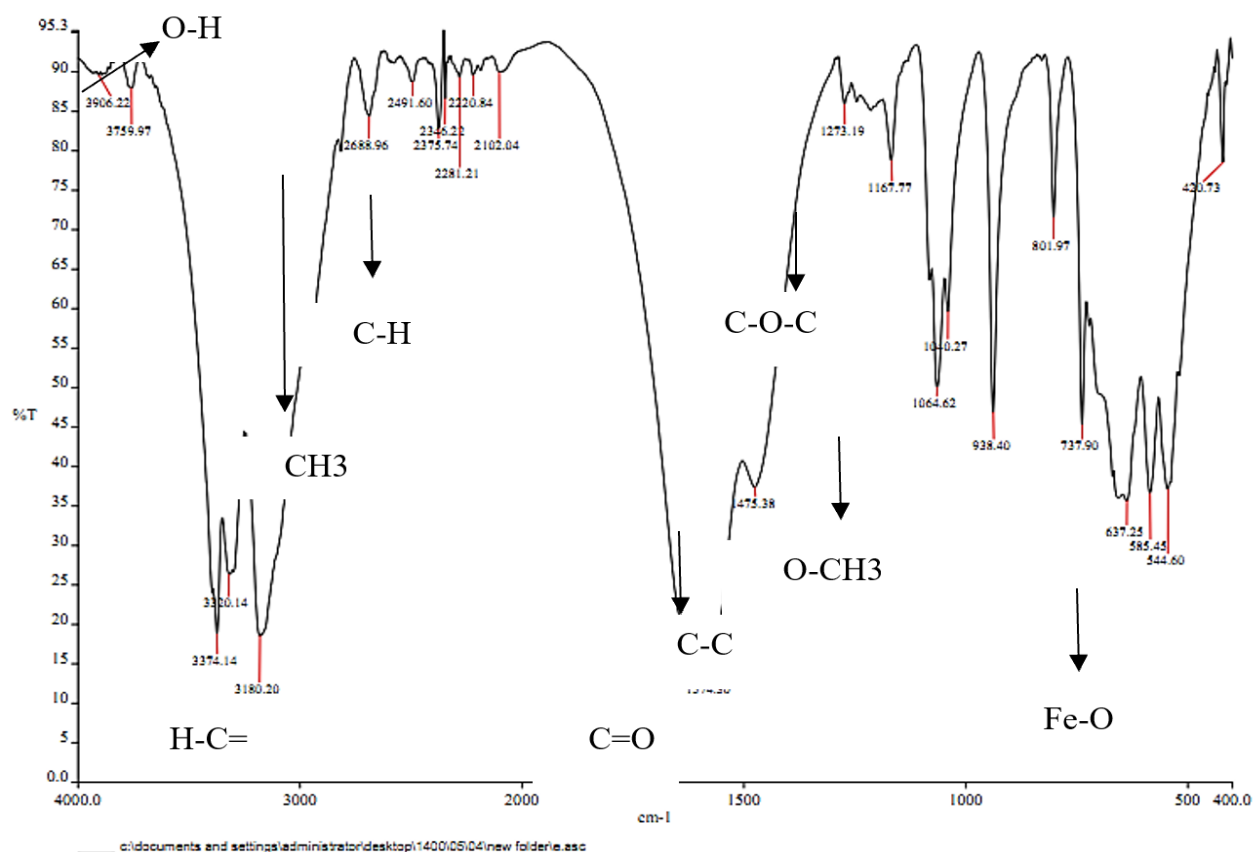
Fig. 1 FT-IR spectra of SNPsGQD@ \beta -cyclocital.
