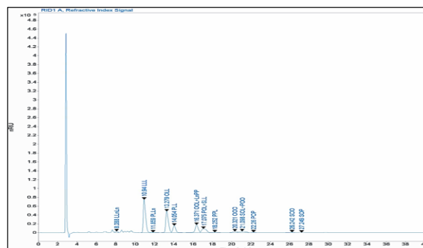
Fig. 2 HPLC chromatogram of the amount of triglycerides in oils made from Gundelia species seeds.
