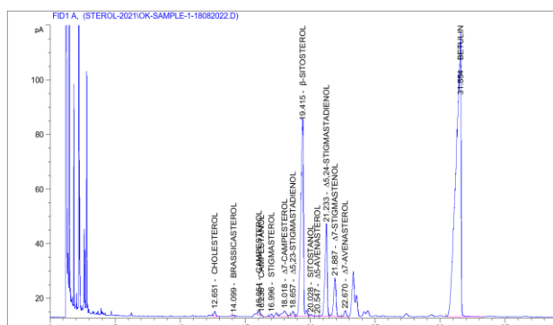
Fig. 3 GC chromatogram of sterol content of oils obtained from seeds of Gundelia species.
