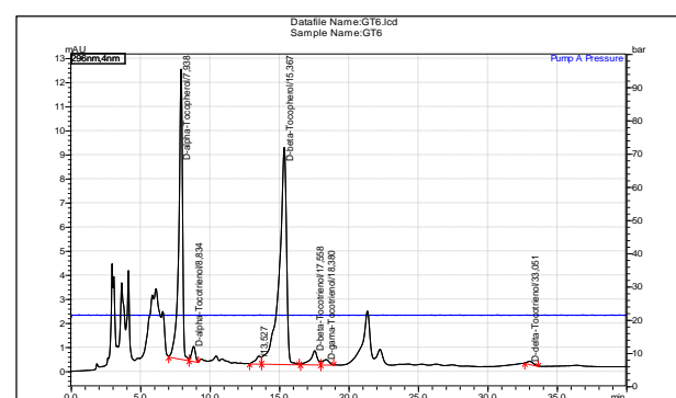
Fig. 4 HPLC chromatogram of tocopherol and tocotrienol (tocols) content of oils made from the seeds of Gundelia species.
