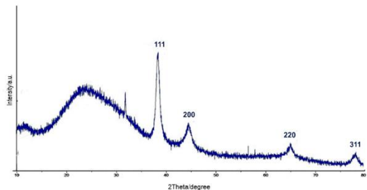
Fig. 4 XRD spectrum of gold nanoparticles synthesized by essential oils of Salvia rosmarinus
