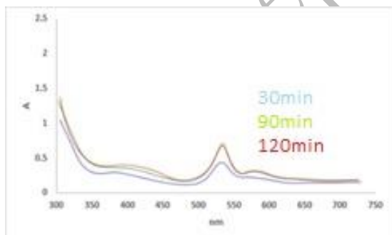
Fig. 2 UV-VIS spectrum of gold nanoparticles synthesized with Salvia rosmarinus essential oil
