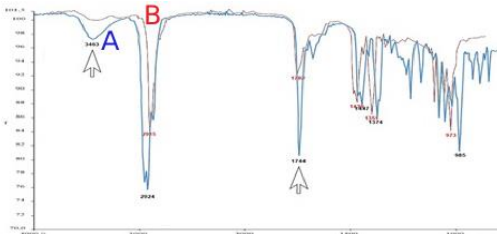
Fig. 3 FT-IR spectrum obtained from essential oils (A) of Salvia rosmarinus and Au-NPs(B)
