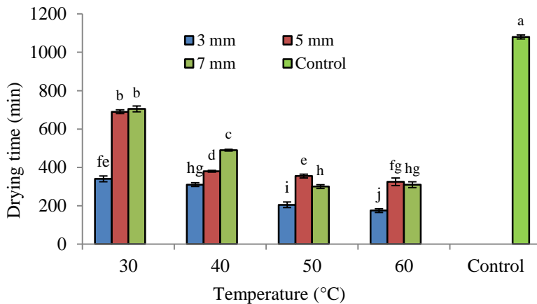
Fig. 5 Interaction of temperature and thickness of root slices of Euphorbia condylocarpa for drying kinetics. (Non-similar letters means significant difference at p < 0.01 ).
