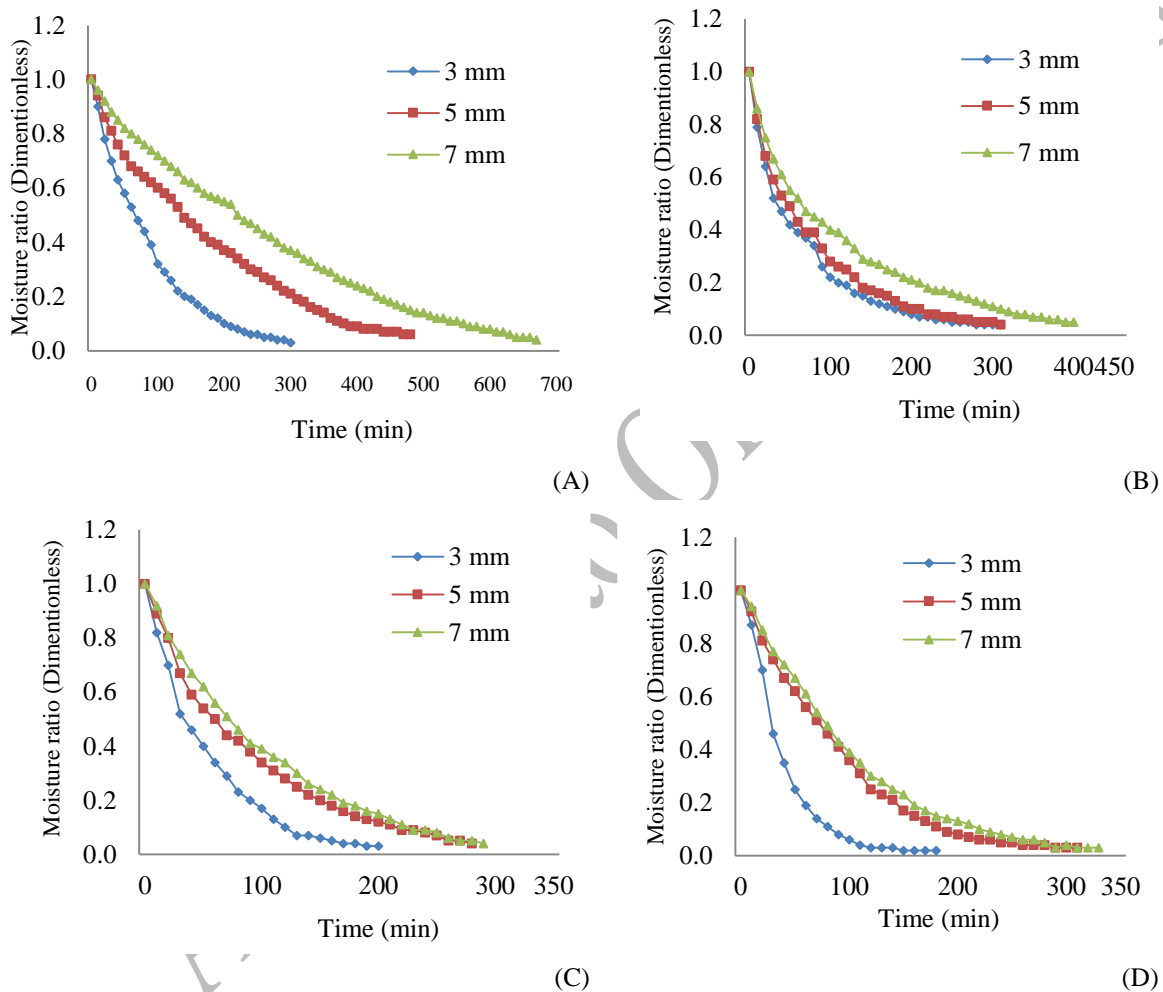
Fig. 4 The moisture ratio of Euphorbia condylocarpa root slices during drying at air velocity of 0.5 m. s -1 , thicknesses of 3, 5, and 7 mm and temperatures of A) 30 °C, B) 40 °C, C) 50 °C and D) 60 °C.
