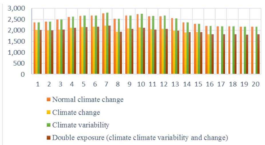
Figure 2. Wheat crop cultivation area due to climate change
