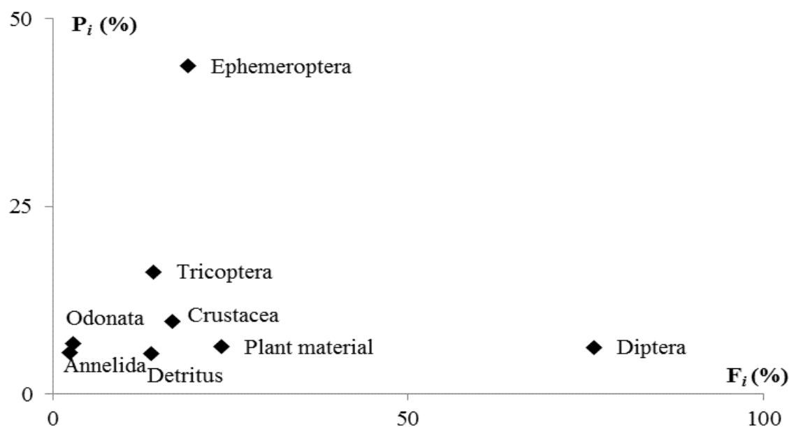
Figure 5: Modified Costello feeding strategy diagram for Gobio bulgaricus in the Istranca Stream. Prey-specific abundance ( P_i ) plotted against frequency of occurrence ( F_i ) of food items in the diet of the species.
