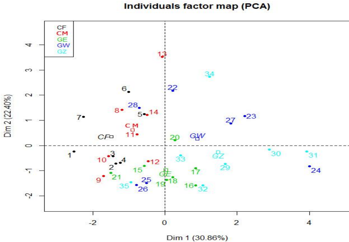
Figure 5: Principal component analysis of sampling sites shows separation between the Caspian (CF, CM) and Gorgan (GW, GE, GZ) sites.
