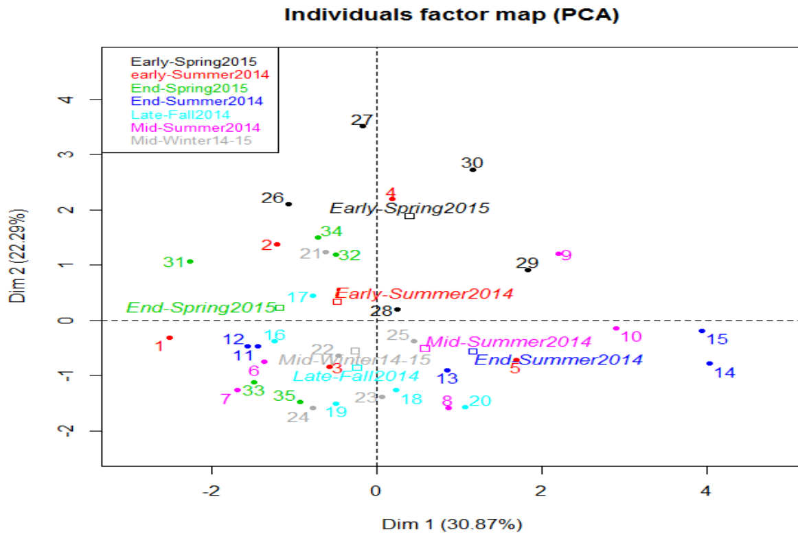
Figure 6: Principal Component Analysis of seven sampling times indicating the particle composition correlations.
